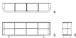
Interior view 4: plan 5: front 6: side Vista interna 4: superior 5: frontal 6: lateral
