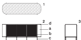
a.wood finish b.front finish c.metal finish d.stone top
